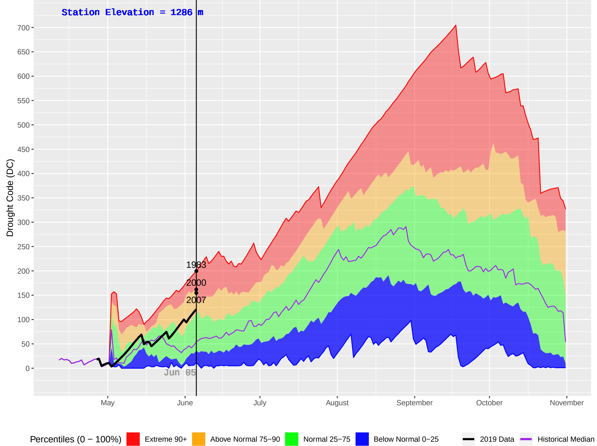
CURWEN CREEK (352) : Historical (1979–2018) and Current (2019) Daily Drought Code (DC)
