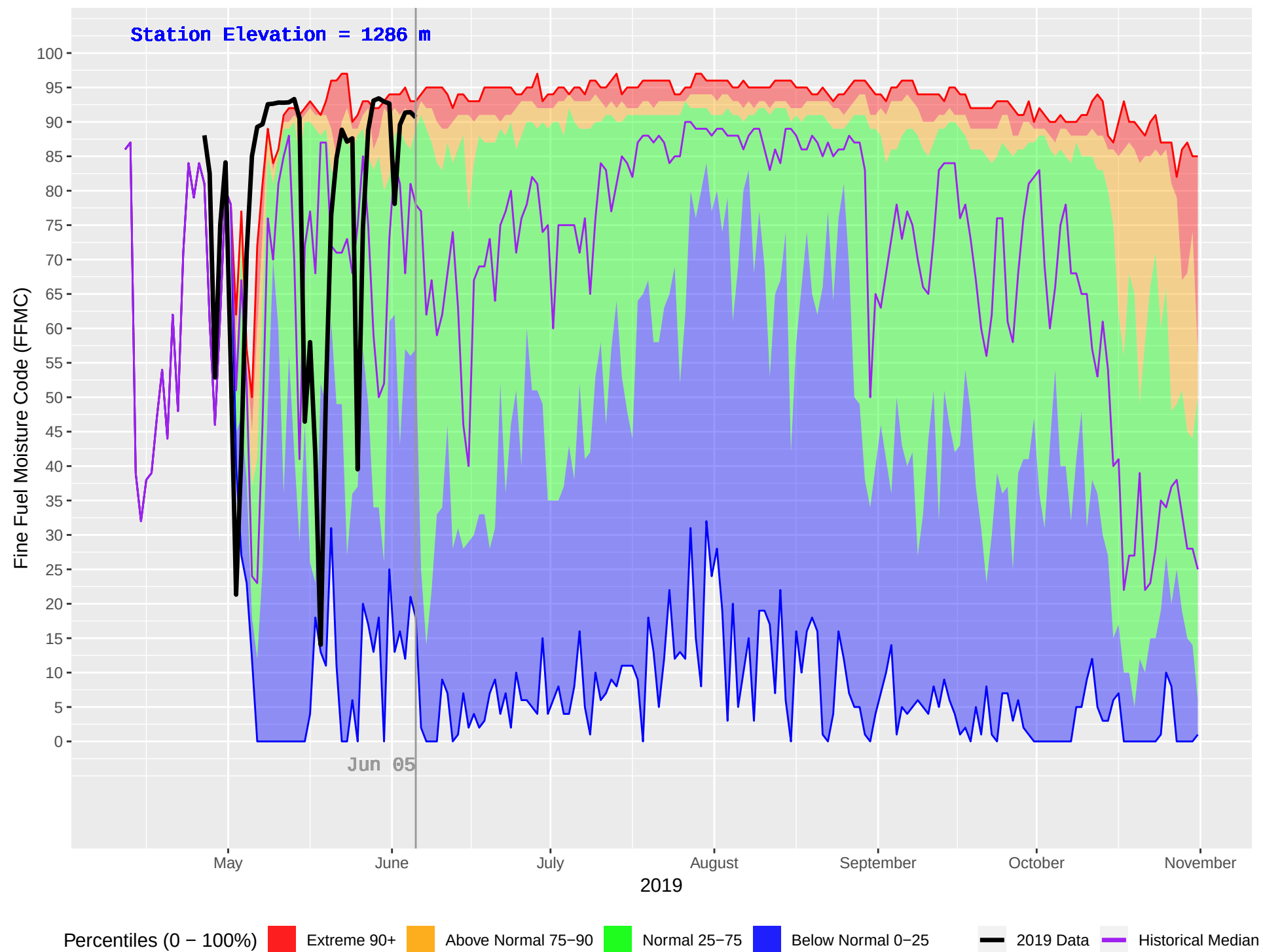
CURWEN CREEK (352) : Historical (1979–2018) and Current (2019) Daily Fine Fuel Moisture Code (FFMC)
