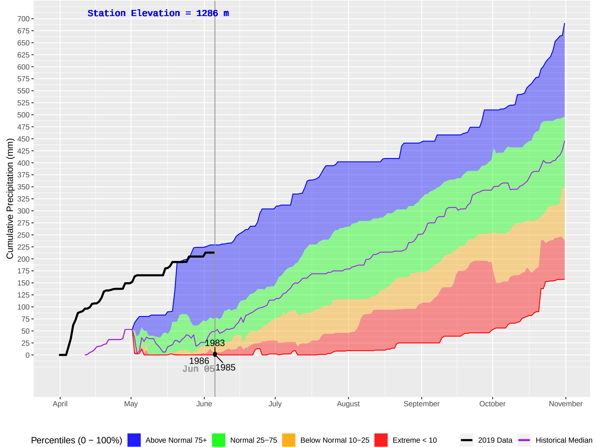
CURWEN CREEK (352) : Historical (1979–2018), Current (2019) Daily Cumulative Precipitation
