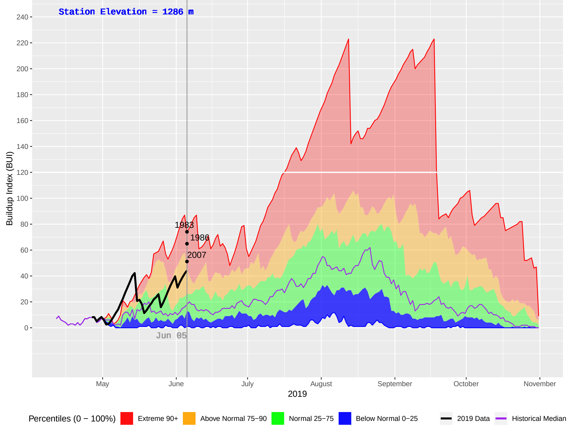
CURWEN CREEK (352) : Historical (1979–2018), Current (2019) Daily Buildup Index (BUI)
