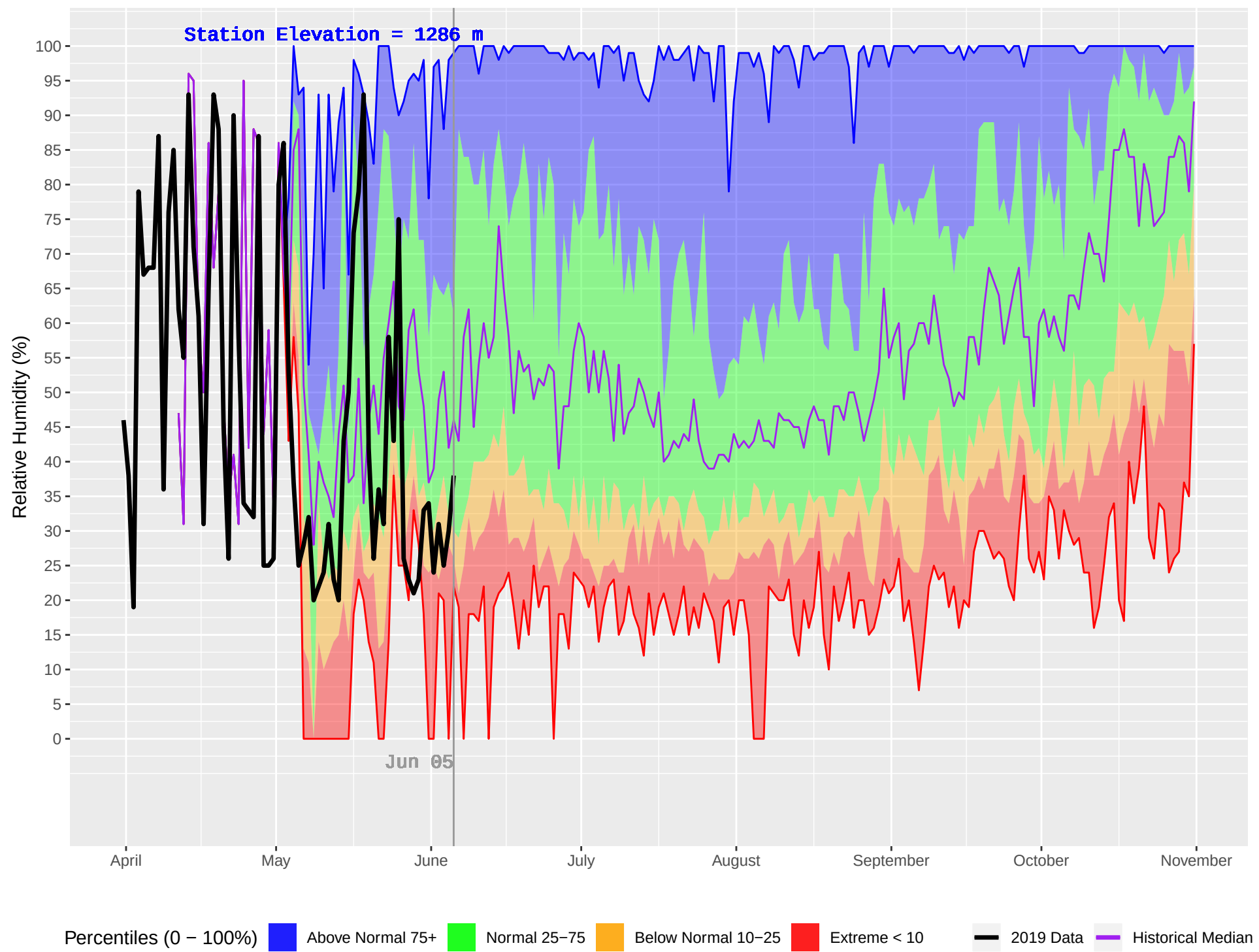
CURWEN CREEK (352) : Historical (1979–2018) and Current (2019) Daily Relative Humidity
