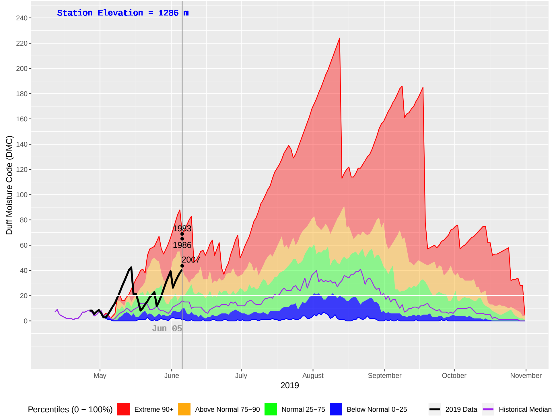
CURWEN CREEK (352) : Historical (1979–2018), Current (2019) Daily Duff Moisture Code (DMC)
